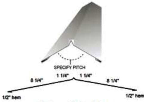
Universal Ridge Cap
