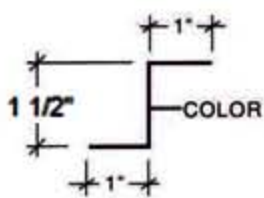
Z - Flashing
