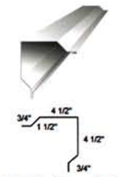
Outside Corner Trim
