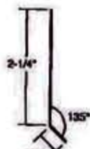
Cleat
