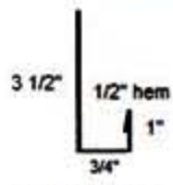
3/4" J - trim
