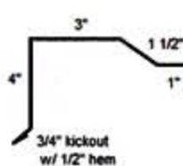
Rake Trim (High Rib Residential)
