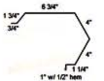
Rake Trim (Industrial)
