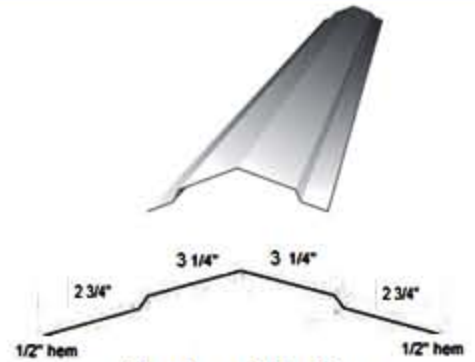
Step Down Ridge Cap
