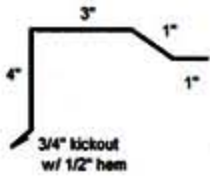
Rake Trim ( Eagle Rib Residential)
