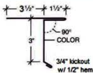
*** Specify Roof Slope Extended Eave Trim
