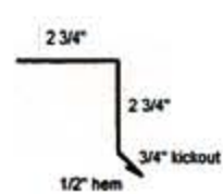
Drip Trim
